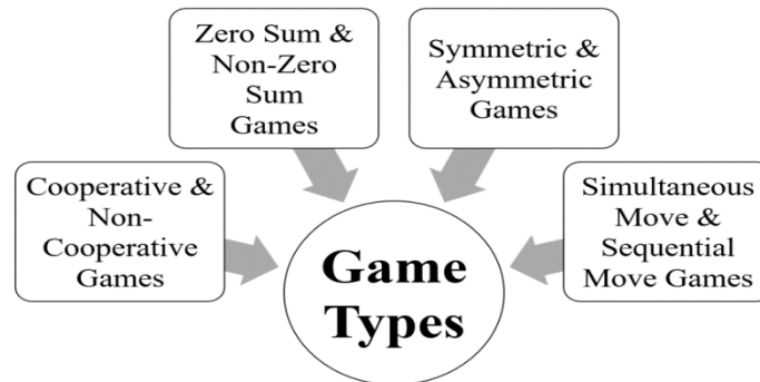
Fig.4.Game Theory Types
